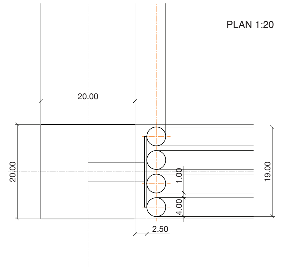
DETAIL 1:5
