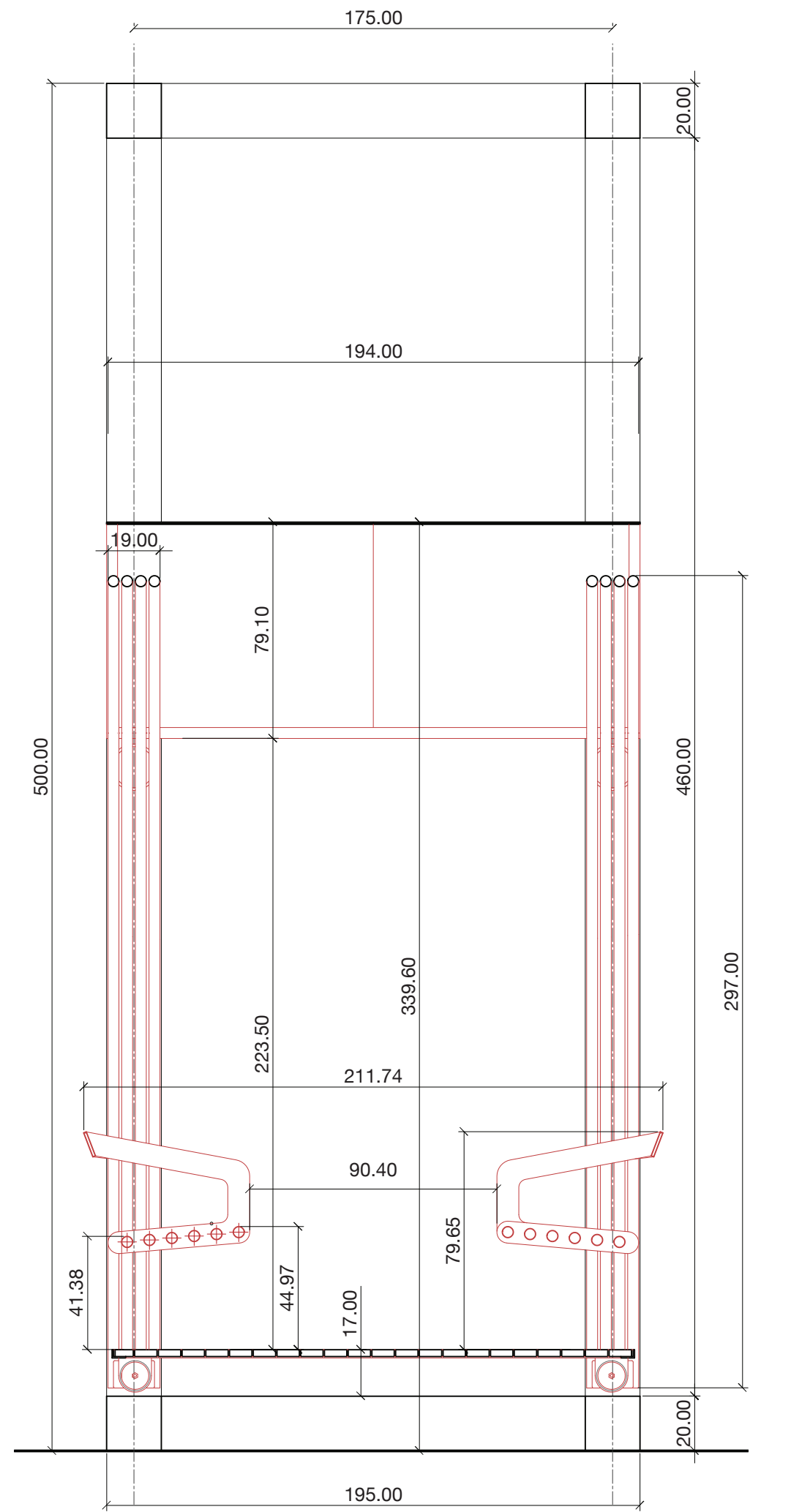
SECTION 1 1:20
