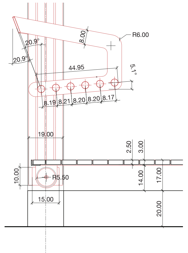
DETAIL BENCH 1:10
